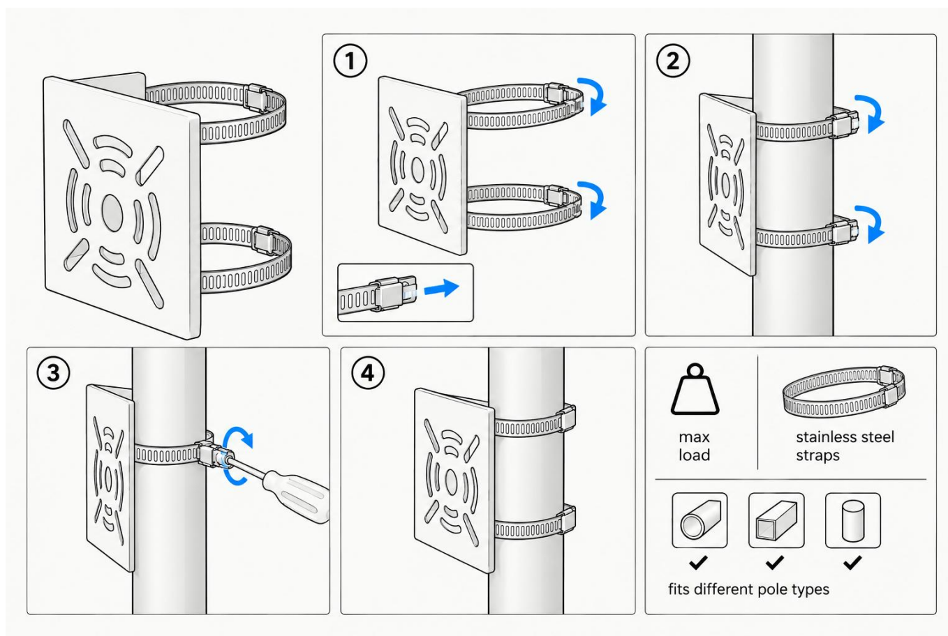
Fig.1. Assembly
